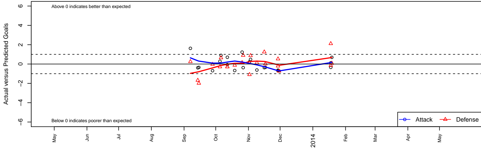
Anaheim Surf White G00 Dots are actual minus expected GF (blue circles) and GA (red triangles). Blue line is smoothed change in attack strength. Red is smoothed change in defense strength.
